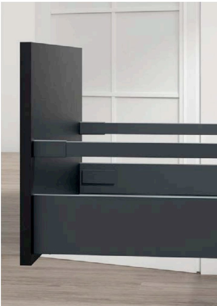
83mm Internal Drawer Front Fixing
